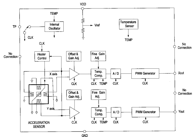
MXD7202G/H/M/N FUNCTIONAL BLOCK DIAGRAM
